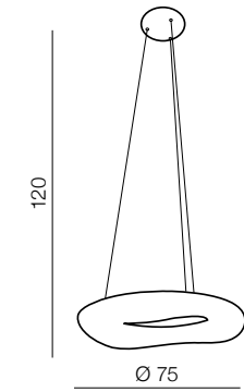
Donut Pendant 75 LED AZ2060 LED 80W 3000K 6800lm acryl dimmmable
